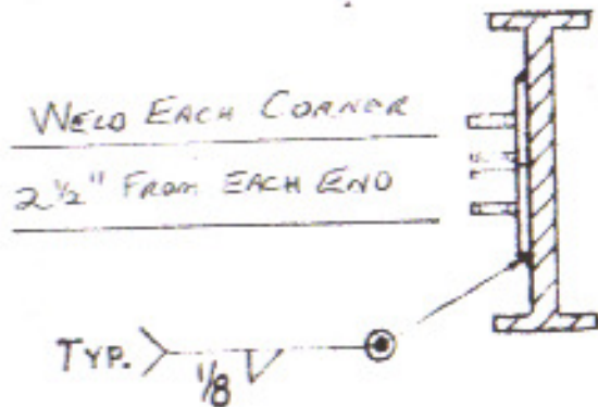
DETAIL 2 BEAM MOUNTING VERTICAL SURFACE
