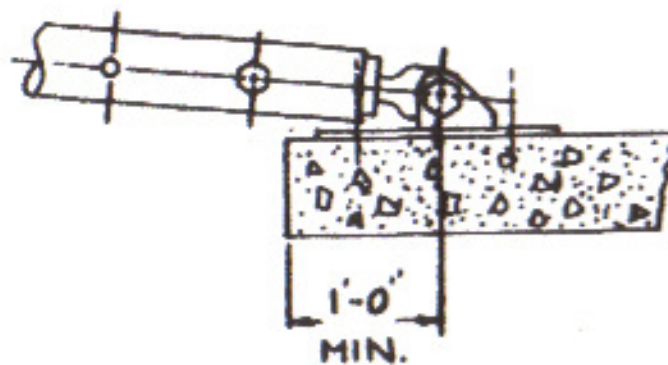
DETAIL 1 FLOOR MOUNTING (HORIZONTAL SURFACE)
